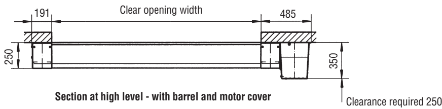
In-line motor option
