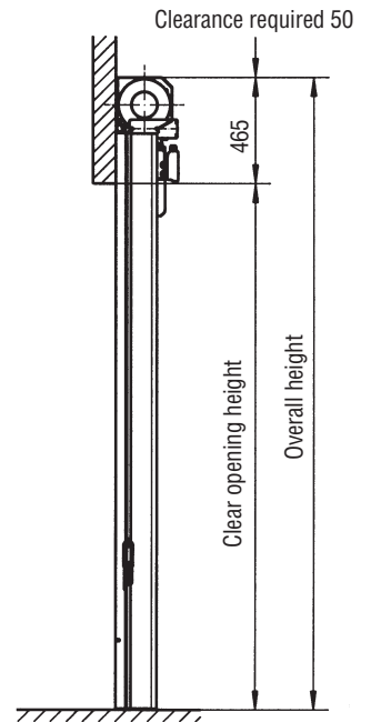
Vertical section - without barrel and motor cover
