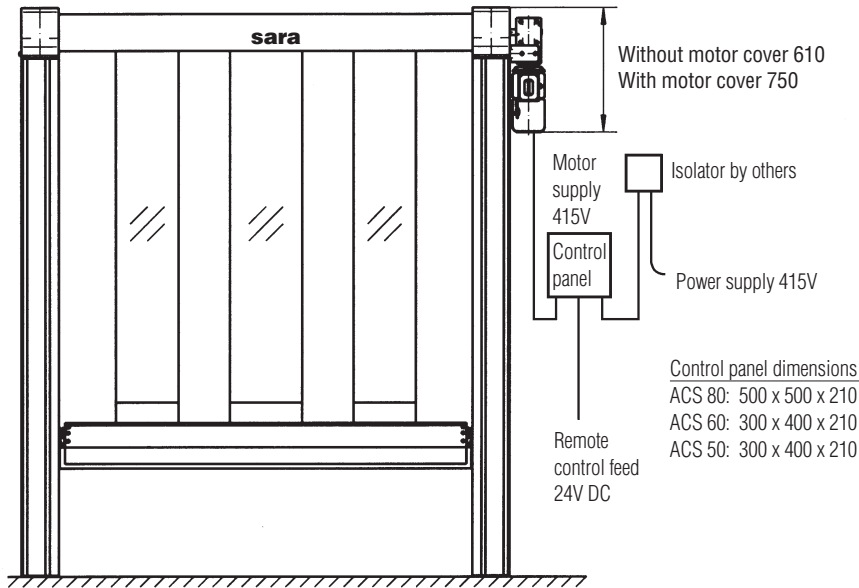
Elevation - direct drive
