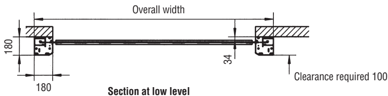
Section at low level
