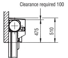
Vertical section - with barrel and motor cover
